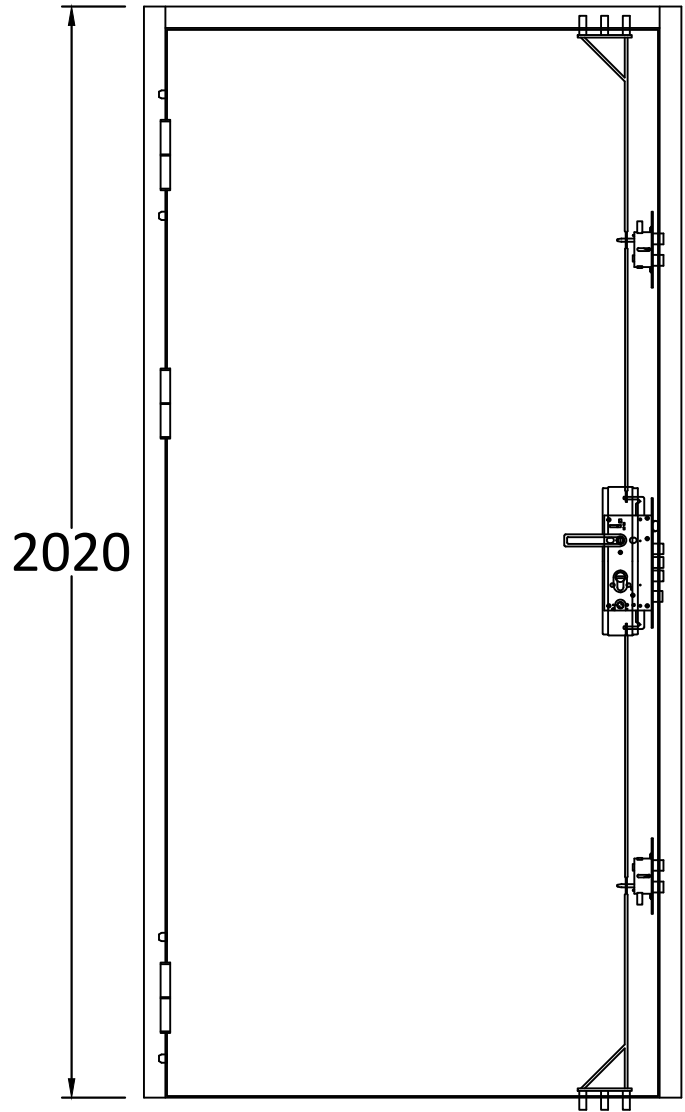
OUTSIDE VIEW 995
